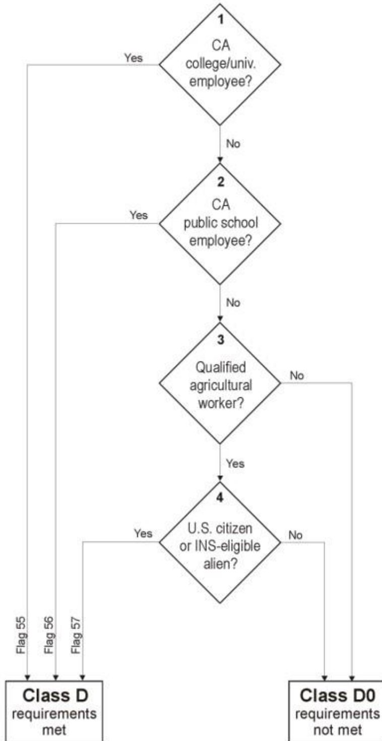
Figure 4. Flowchart for Residency Area D Logic Residency Status Calculation
